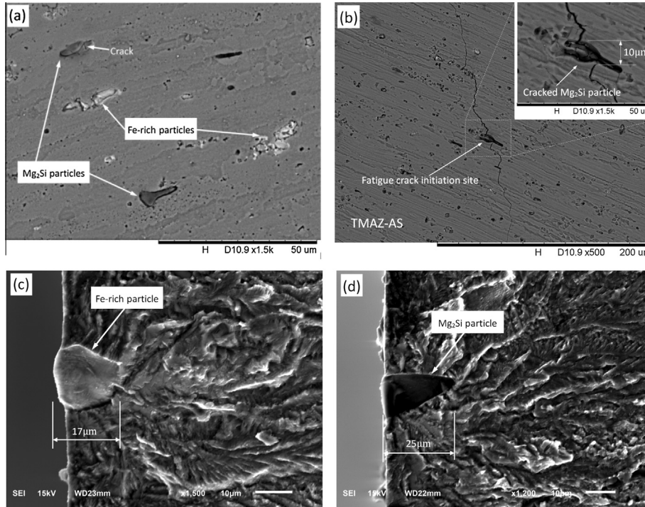
Fig. 8. Types of particles distributed at the TMAZ. (a) Morphological characteristics before the fatigue loading showing pre-existed cracks; (b) fatigue crack initiation from a cracked Mg_2Si particle ( N_f = 1.46 \times 10^6 cycles, \sigma_b = 90 MPa); (c) fatigue crack initiation induced by a Fe-rich particle ( N_f = 4.38 \times 10^6 cycles, \sigma_b = 80 MPa); (d) fatigue crack initiating from a Mg_2Si particle ( N_f = 2.59 \times 10^6 cycles, \sigma_b = 80 MPa).
